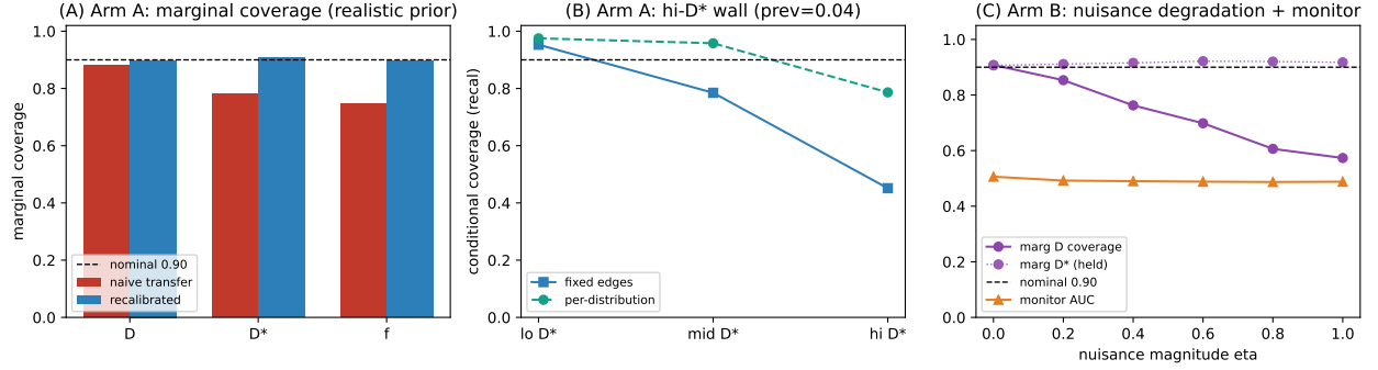
Figure 10: Realism cohort (realistic synthetic; no in-vivo coverage claim). (A) Arm A – marginal coverage under a realistic correlated/skewed prior: naive transfer of the uniform-calibrated predictor breaks, within-distribution recalibration restores nominal coverage. (B) Arm A – recalibrated high- D^* tercile coverage on fixed physical boundaries vs. per-distribution quantiles; the wall persists in both, concentrated in a clinically rare high- D^* tail (fixed prevalence \approx 0.05 ). (C) Arm B – the measurement-noisance envelope: marginal D coverage degrades with the nuisance magnitude (the wider D^* interval is held) while the deployment monitor’s AUC stays at chance, a silent channel. Seed-20260613 panel (across-seed [5,95] bands quoted in text); from results/realism_report.txt.
