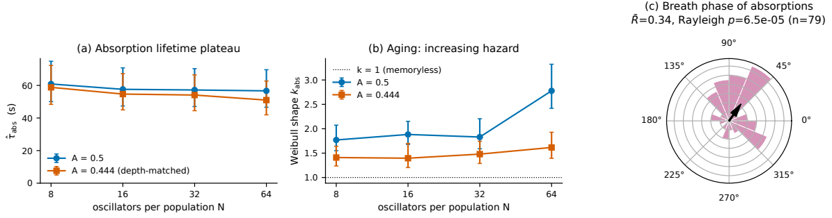
Figure 10: Robustness at \beta = 0.10 . (a) Absorption lifetime \hat{\tau}_{\text{abs}}(N) is flat in N at both the post-homoclinic corner A = 0.5 and the depth-matched A = 0.444 . (b) Censored-Weibull shape k_{\text{abs}}(N) stays above the memoryless value k = 1 (aging persists). (c) True-absorption breath phases remain clustered (pooled \bar{R} = 0.34 , Rayleigh p = 6.5 \times 10^{-5} , n = 79 ).
