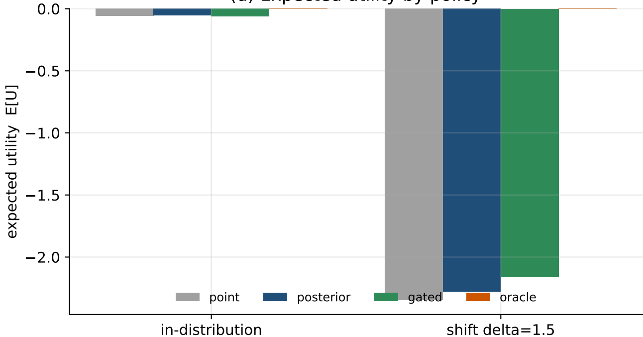
(d) Expected utility by policy
