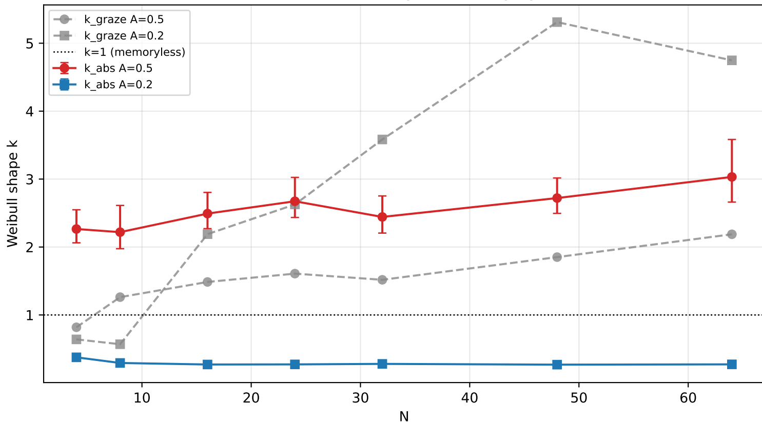
CP3b — aging: Weibull shape k(N) , graze vs absorption-grade ( k > 1 \Rightarrow increasing hazard / aging)
