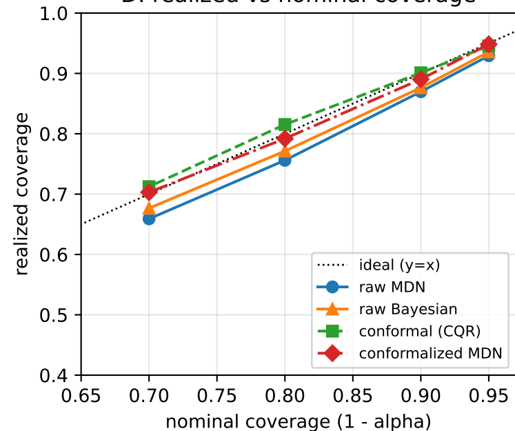
D: realized vs nominal coverage
