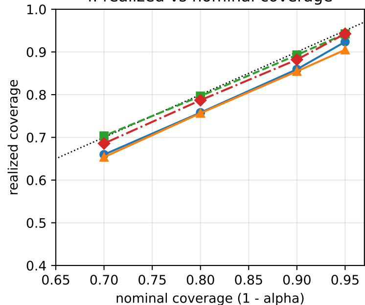
f: realized vs nominal coverage
