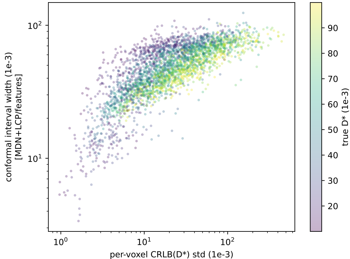
conformal width tracks CRLB (log-log r=0.77 ) intervals widen honestly where D^* is unidentifiable
