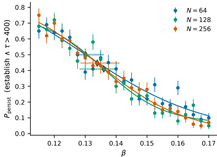
(a) persistence boundary (primary)
