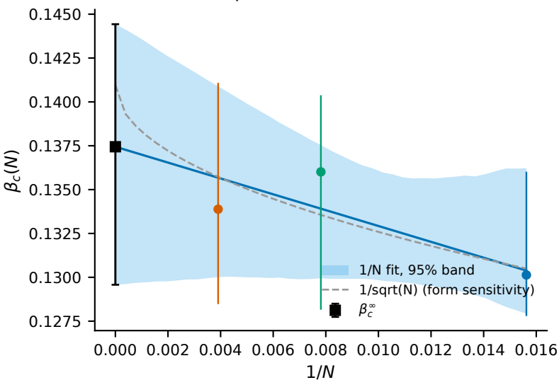
(c) N \rightarrow \infty extrapolation
