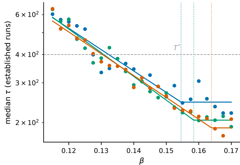
(b) lifetime knee (robustness)
