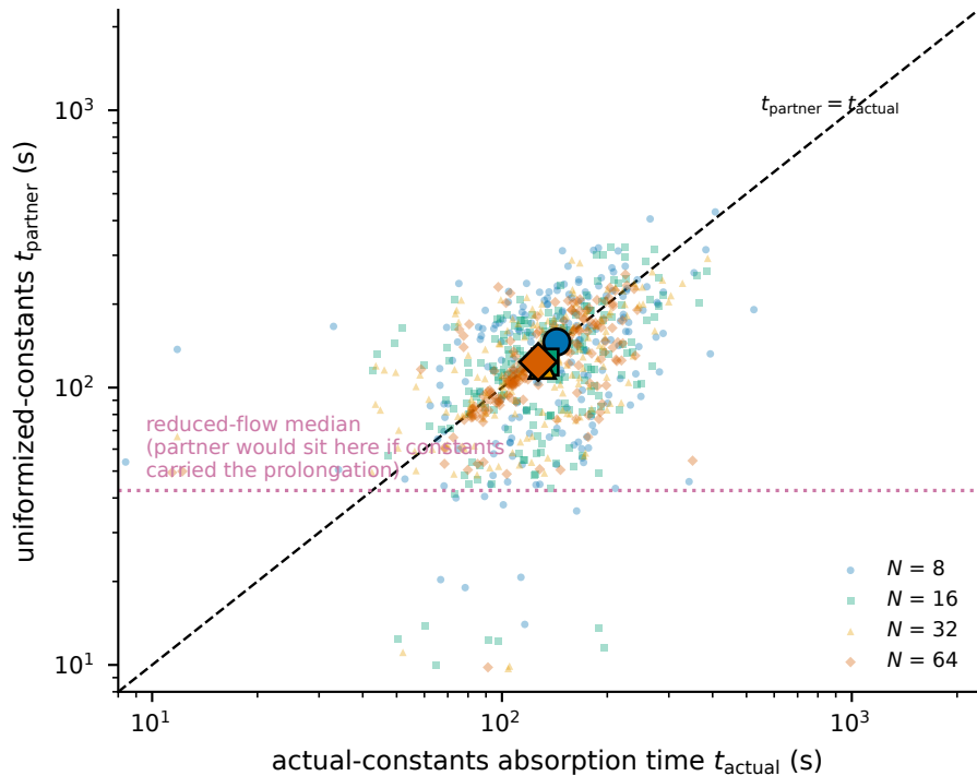
(b) WS-constants decomposition (large = per- N median)
