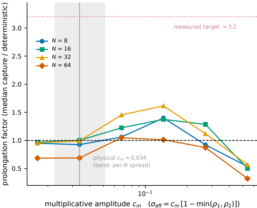
(a) breath-locked multiplicative noise ( N -free amplitude)
