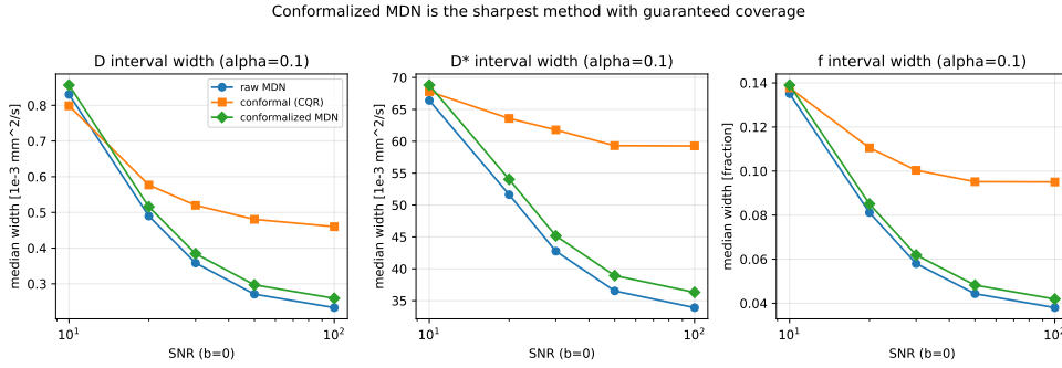
Figure 2: Median interval width vs SNR. Conformalized-MDN is the sharpest method with a guaranteed coverage level.
