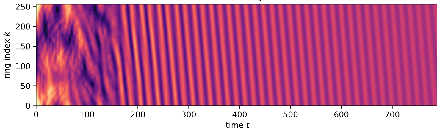
\beta=0.13 , N=256, seed 20266310, \tau=792 : degenerate decay channel (rare, ~2-3%) (chimera dissolves early \rightarrow limbo)
