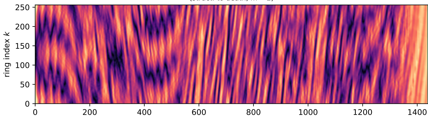
\beta=0.11 , N=256, seed 20265110, \tau=1440 : multi-headed chimera (struct. to death, m^*=2 )
