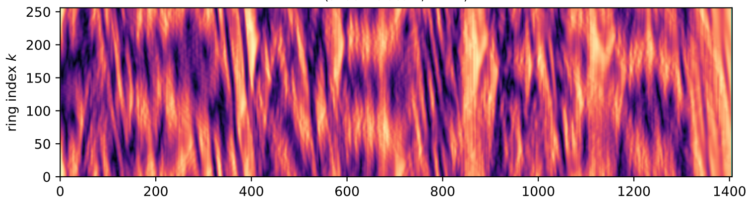
\beta=0.13 , N=256, seed 20266309, \tau=1406 : canonical single-arc chimera (struct. to death, m^*=1 )
