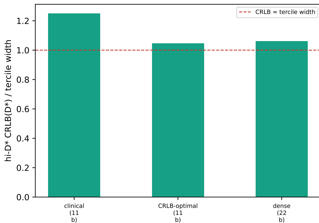
CP1: the resolution wall vs b-scheme
