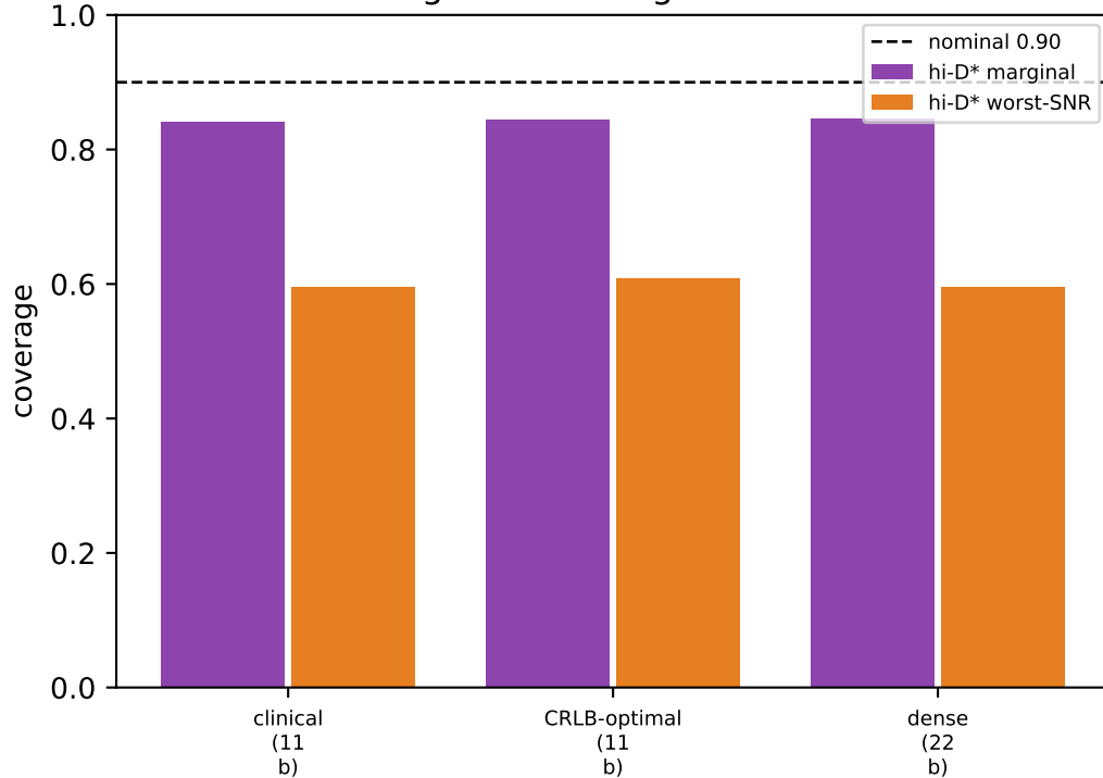
CP1: high-D* coverage vs b-scheme
