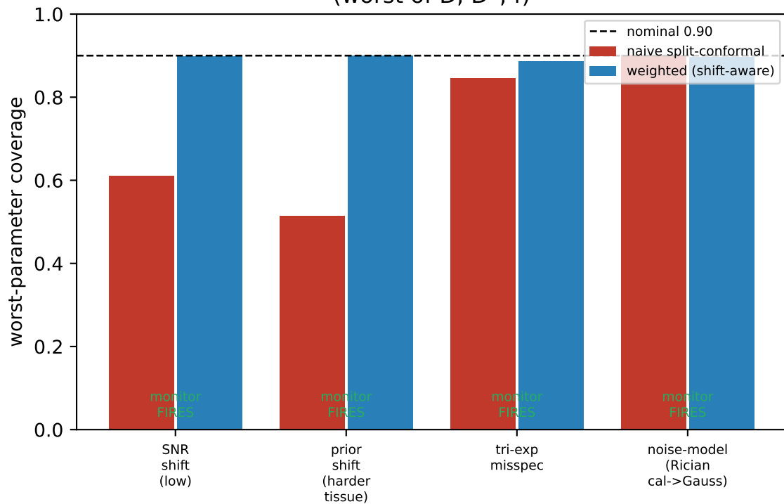
CP0: coverage under exchangeability break (worst of D, D*, f)
