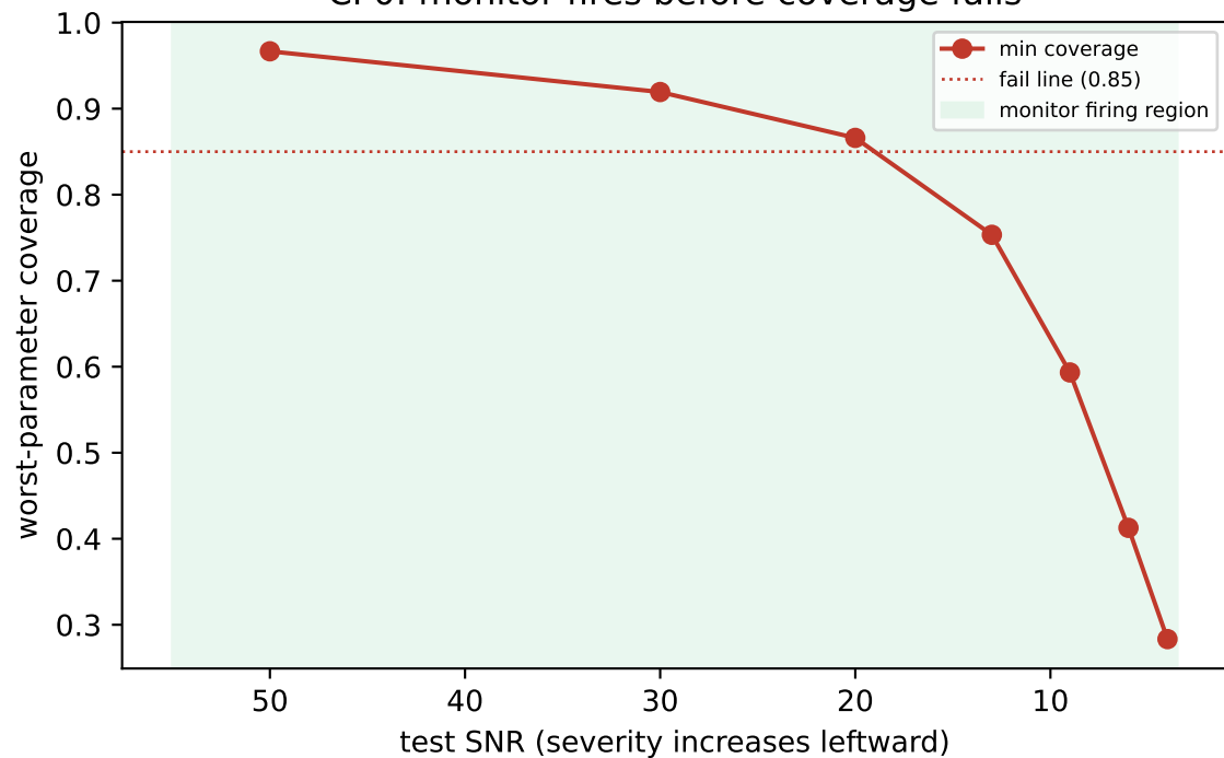
CP0: monitor fires before coverage fails
