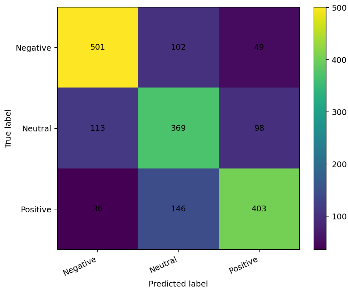
Final Sentiment Model — DistilBERT
