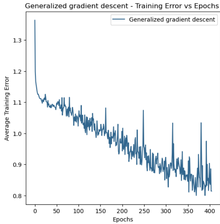
Figure 3: Generalized Delta Rule – Training Error vs Epoch
