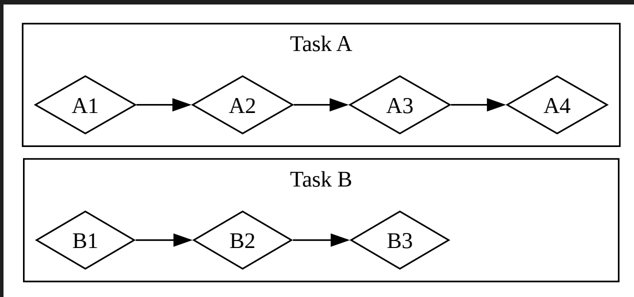
Figure 17-2: A parallel workflow, where work happens on Task A and Task B independently
