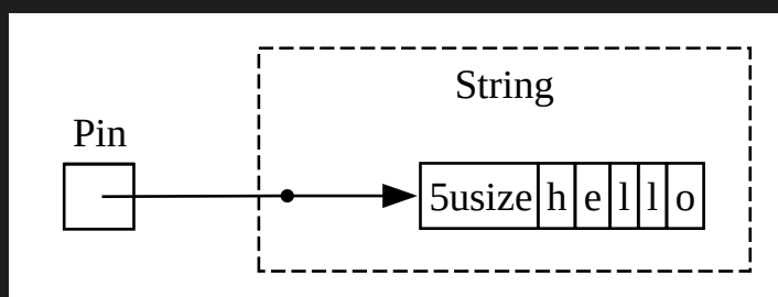
Figure 17-8: Pinning a `String`; the dotted line indicates that the `String` implements the `Unpin` trait and thus is not pinned
