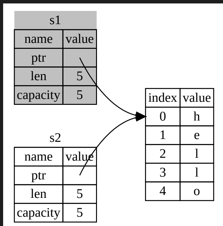
Figure 4-4: The representation in memory after s1 has been invalidated
