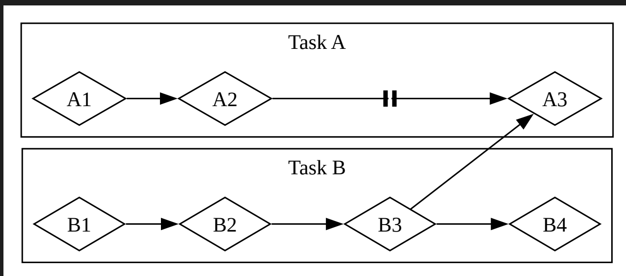
Figure 17-3: A partially parallel workflow, where work happens on Task A and Task B independently until Task A3 is blocked on the results of Task B3.
