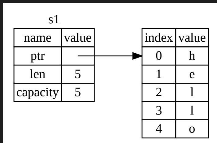
Figure 4-1: The representation in memory of a String holding the value "hello" bound to s1
