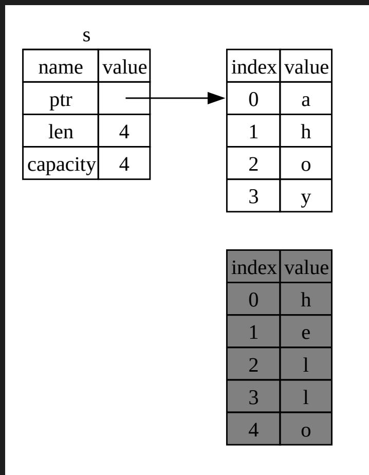
Figure 4-5: The representation in memory after the initial value has been replaced in its entirety
