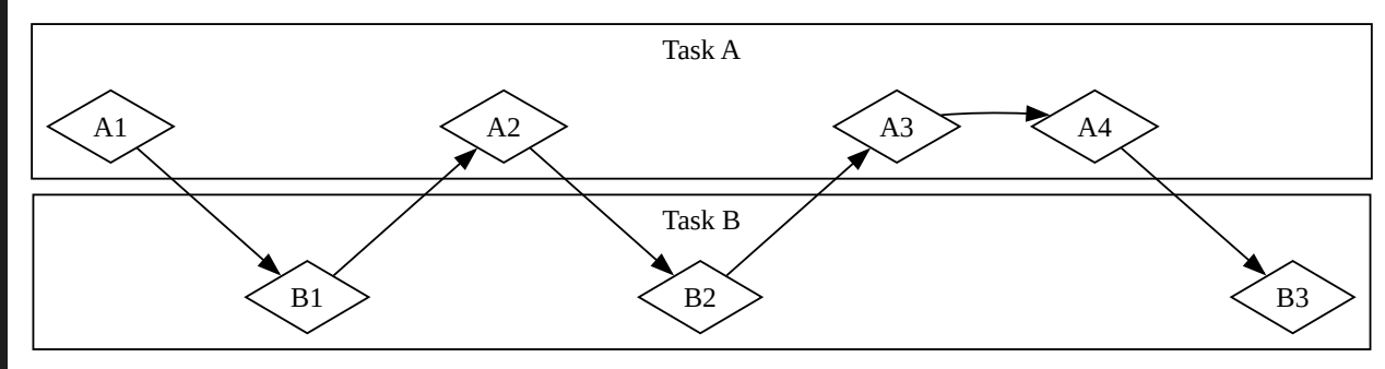
Figure 17-1: A concurrent workflow, switching between Task A and Task B
