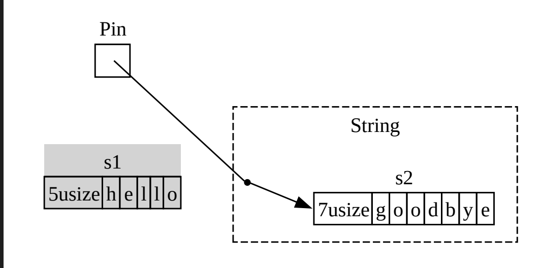
Figure 17-9: Replacing the `String` with an entirely different `String` in memory
