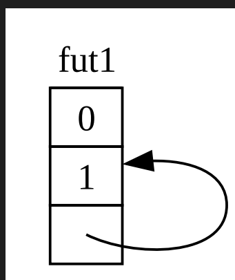
Figure 17-4: A self-referential data type
