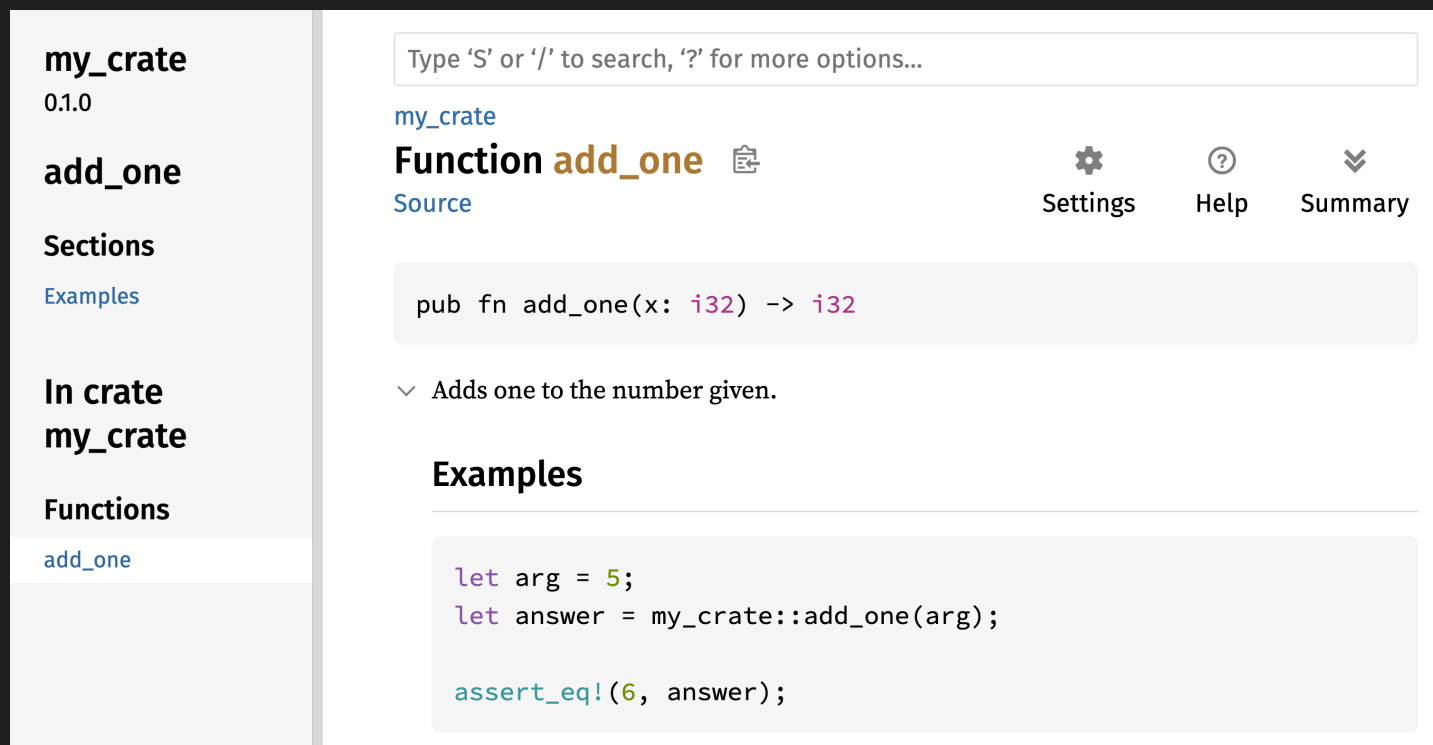
Figure 14-1: The HTML documentation for the add_one function
