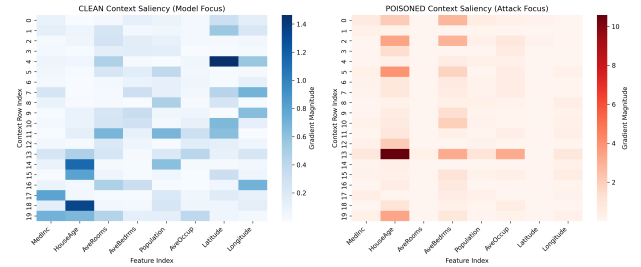
Fig. 1. Gradient Saliency Heatmaps. (Left) The Clean model distributes its attention logically across critical features like Median Income. (Right) The Poisoned model exhibits extreme attention hijacking, fixating aggressively on adversarial artifacts within the context rows.
