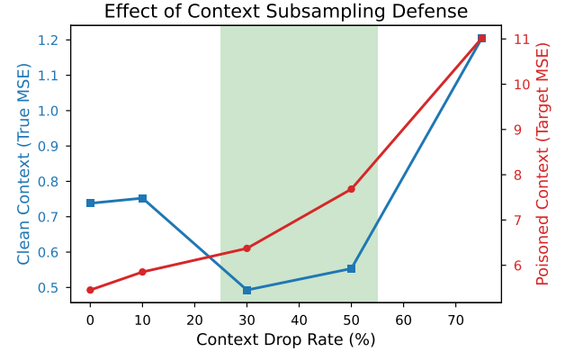
Fig. 3. Effect of Context Subsampling on Adversarial Alignment.
