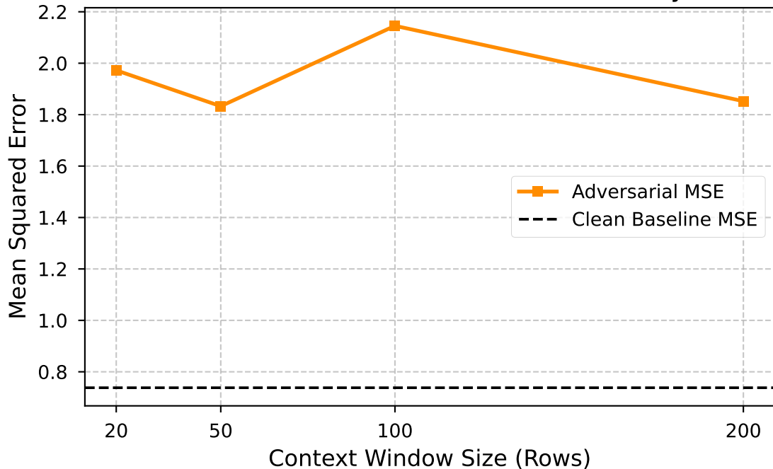
Ablation: Context Size vs. Vulnerability
