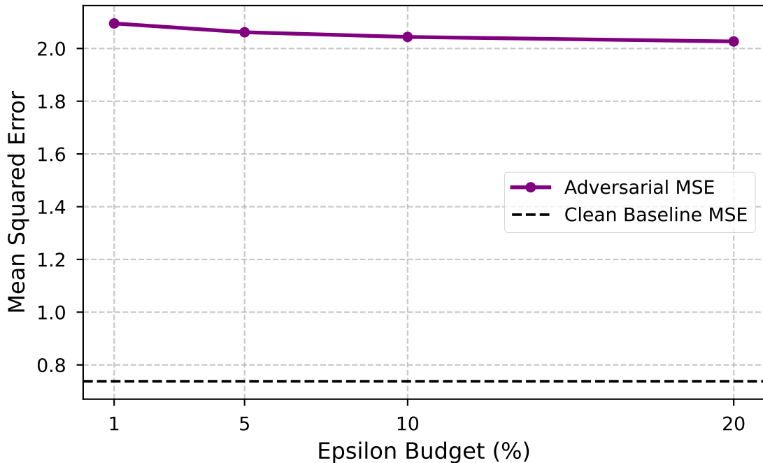
Ablation: Epsilon vs. Vulnerability
