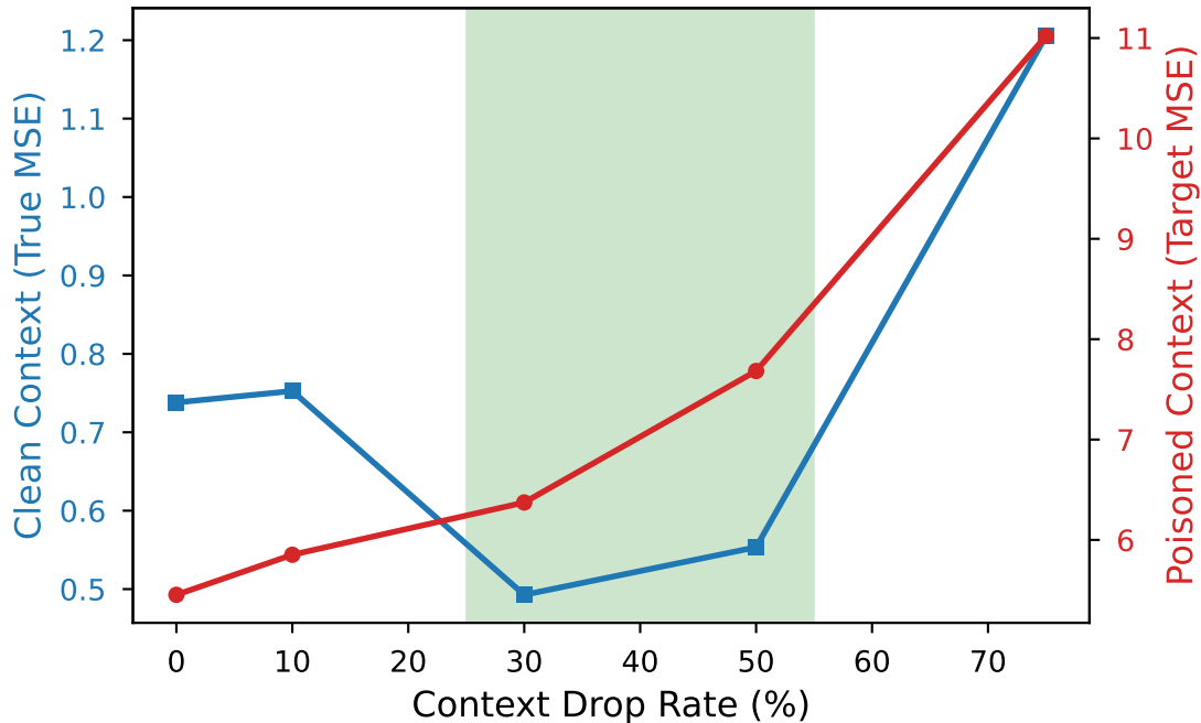
Effect of Context Subsampling Defense
