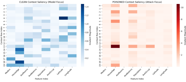
Fig. 1. Gradient Saliency Heatmaps. (Left) The Clean model distributes its attention logically across critical features like Median Income. (Right) The Poisoned model exhibits extreme attention hijacking, fixating aggressively on adversarial artifacts within the context rows.
