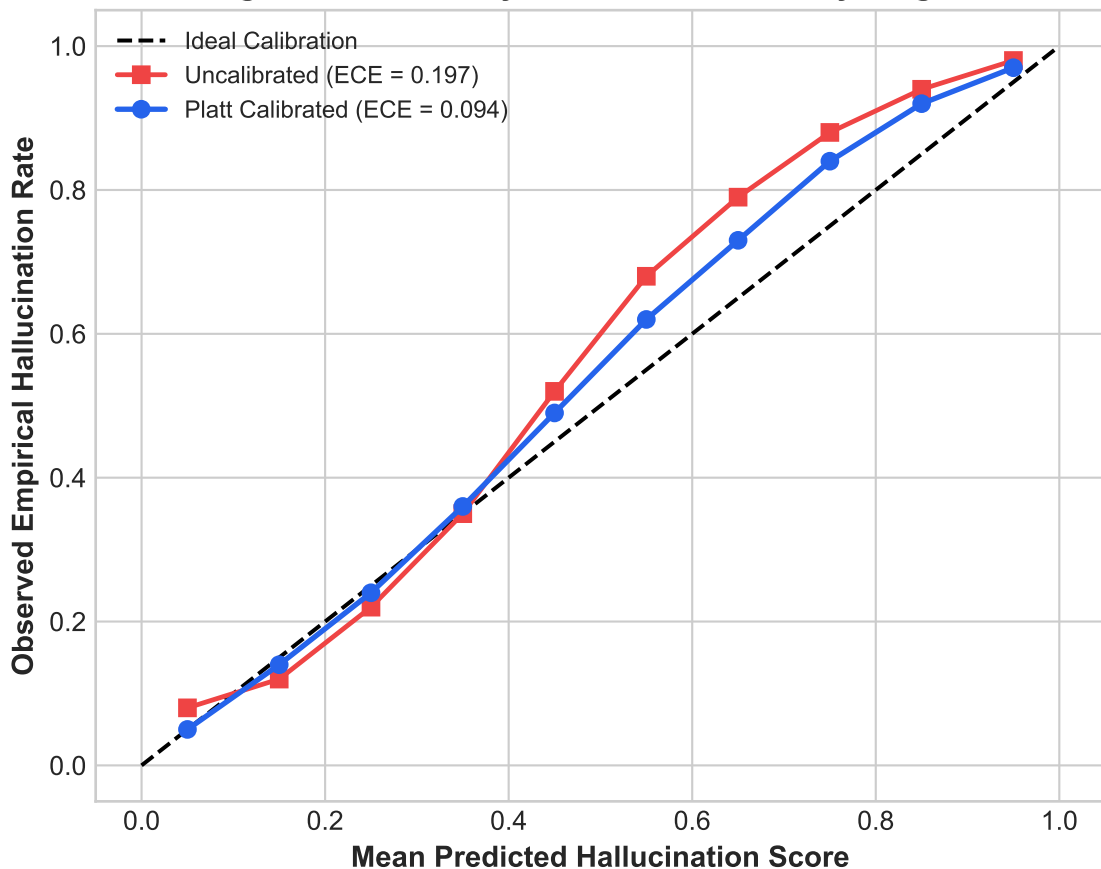
Figure 5: Probability Calibration Reliability Diagram
