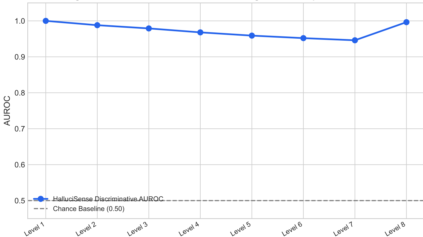
Figure 1: Generalization Ladder Across Progressive Independence Levels
