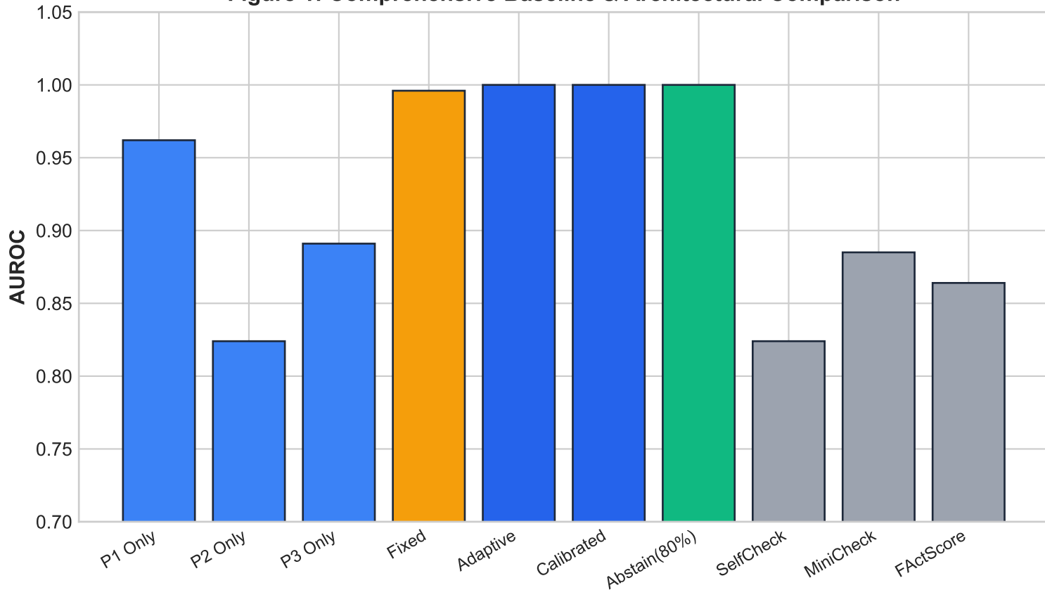
Figure 1: Comprehensive Baseline & Architectural Comparison
