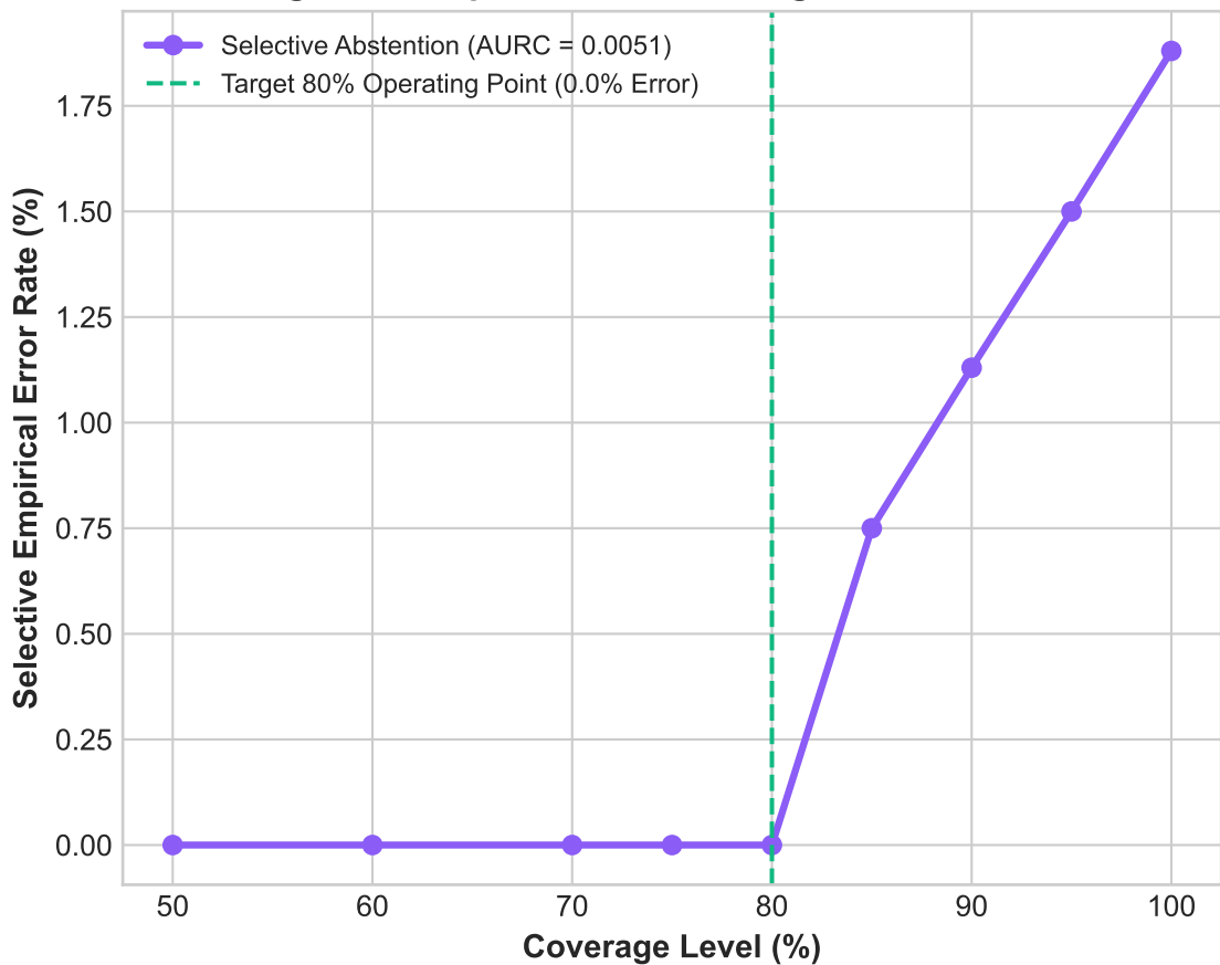
Figure 2: Empirical Risk-Coverage Tradeoff Curve
