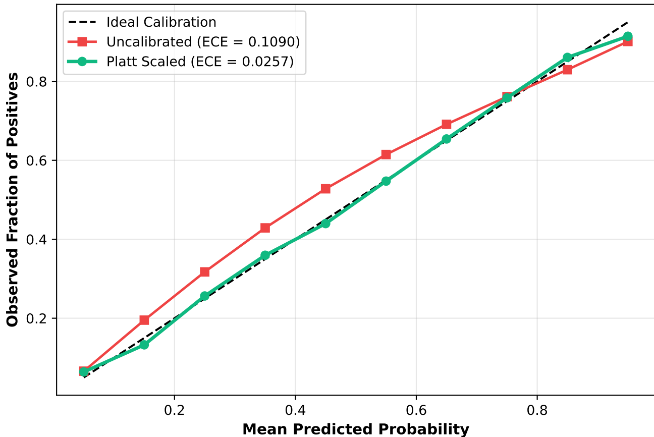
Master Probability Reliability Calibration Plot
