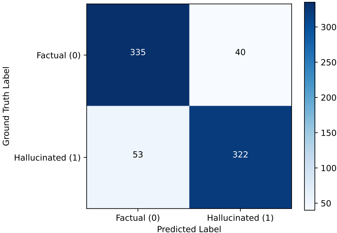
HalluciSense Production Confusion Matrix
