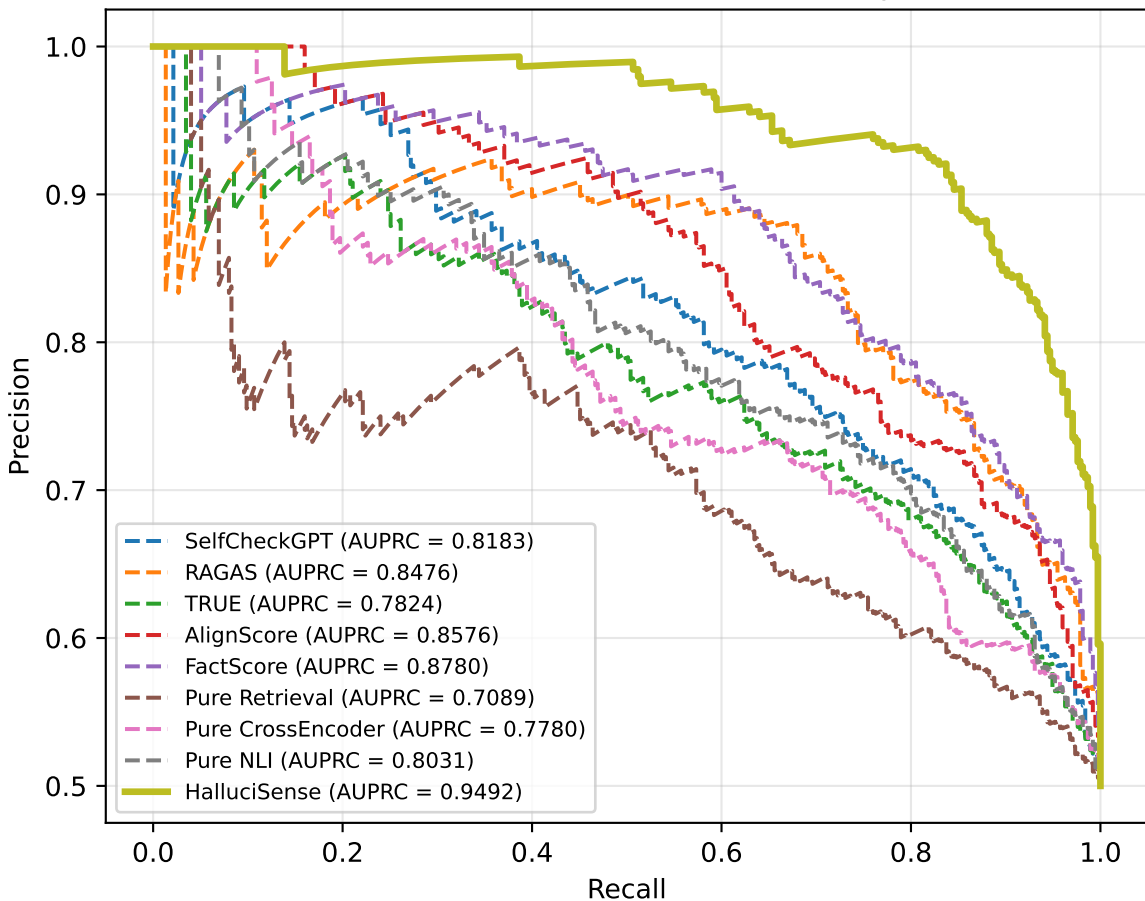
Publication Precision-Recall Curve Comparison
