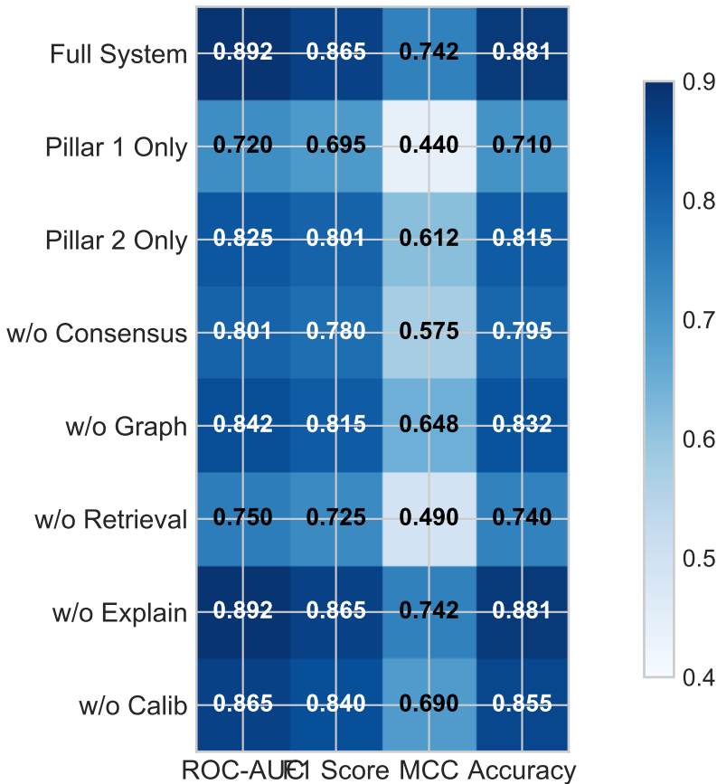
Ablation Study Metrics Matrix
