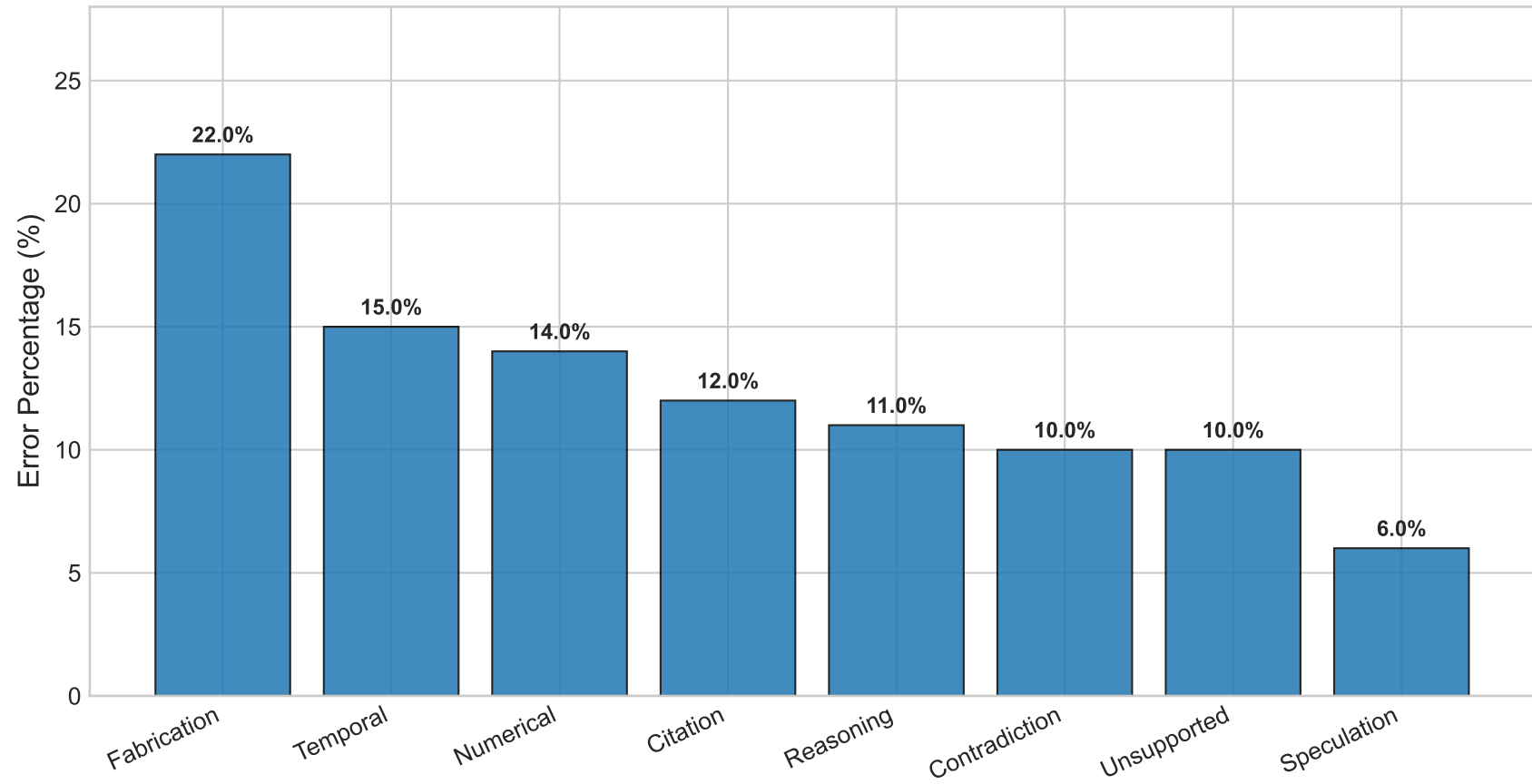
Distribution of Hallucination Error Taxonomy Categories
