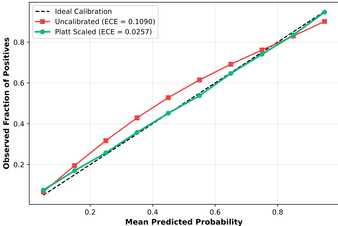
Reliability Diagram — EXP0005
