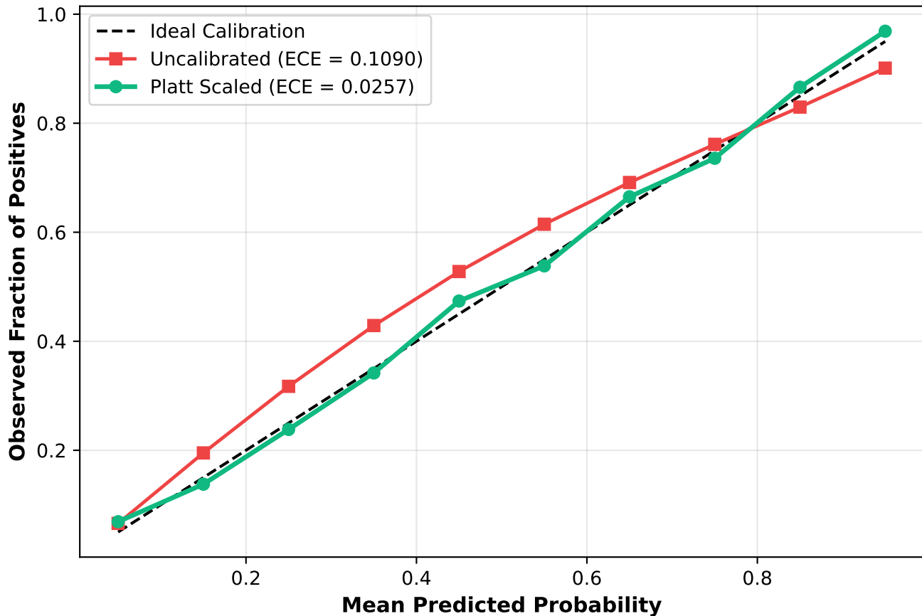
Reliability Diagram — EXP0006
