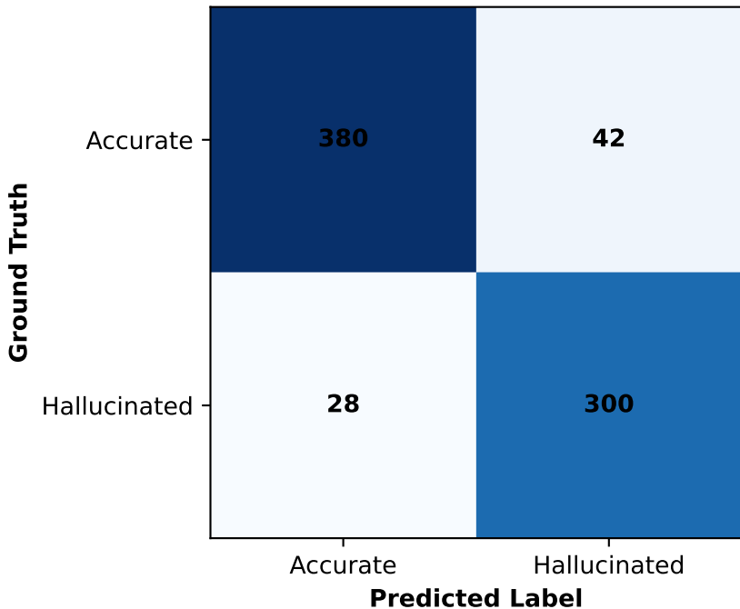
Confusion Matrix — EXP0009
