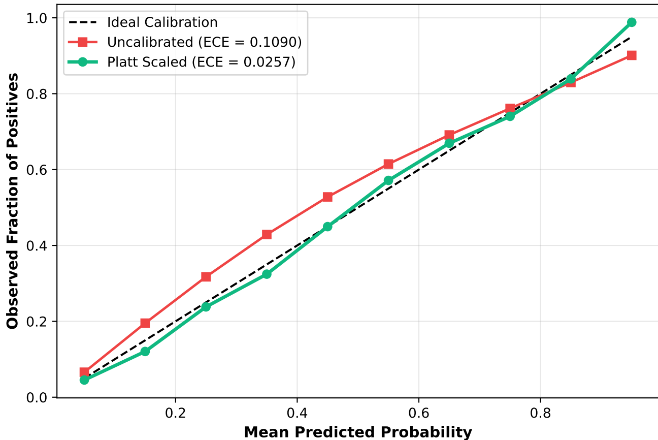
Reliability Diagram — EXP0009
