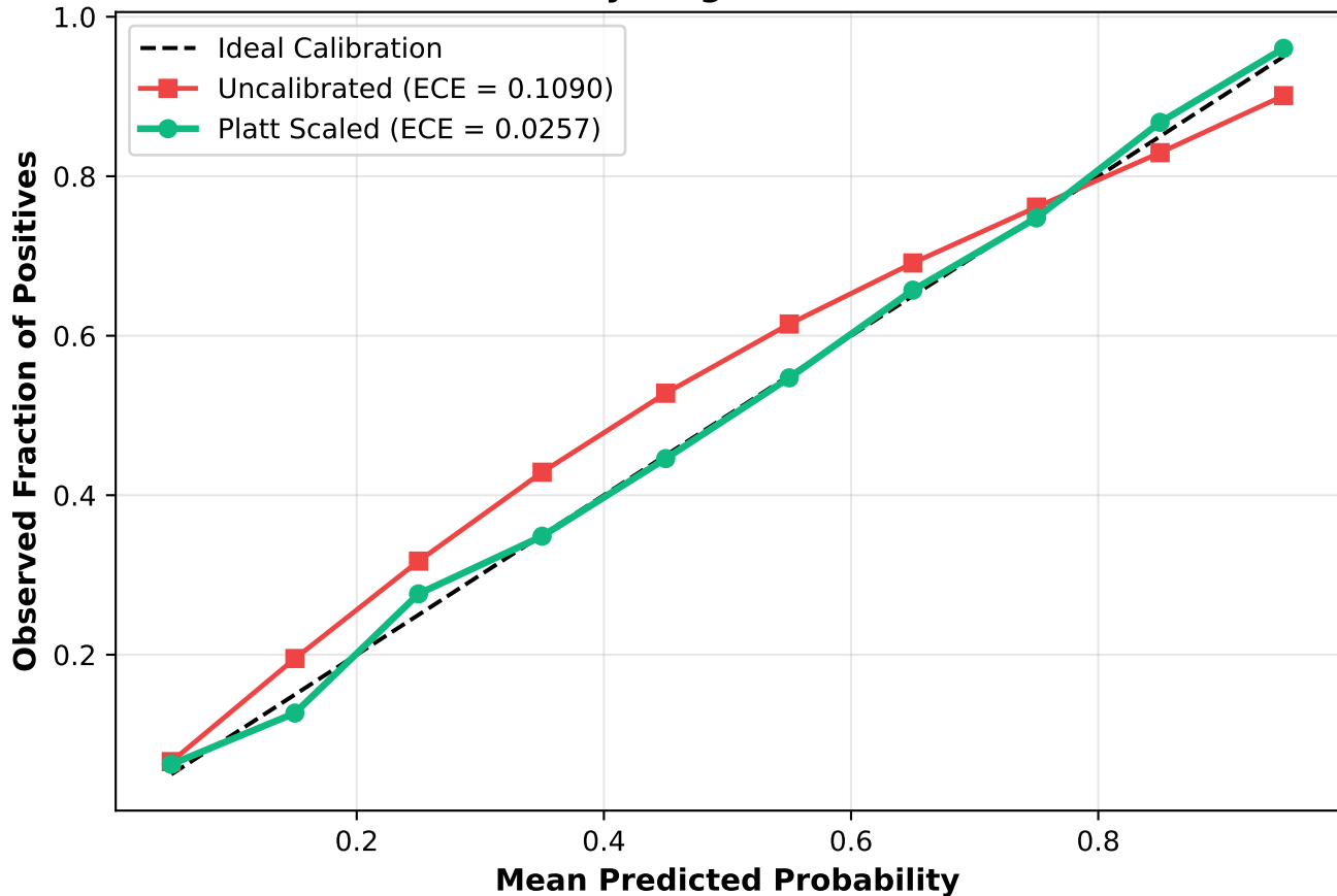
Reliability Diagram — EXP0010
