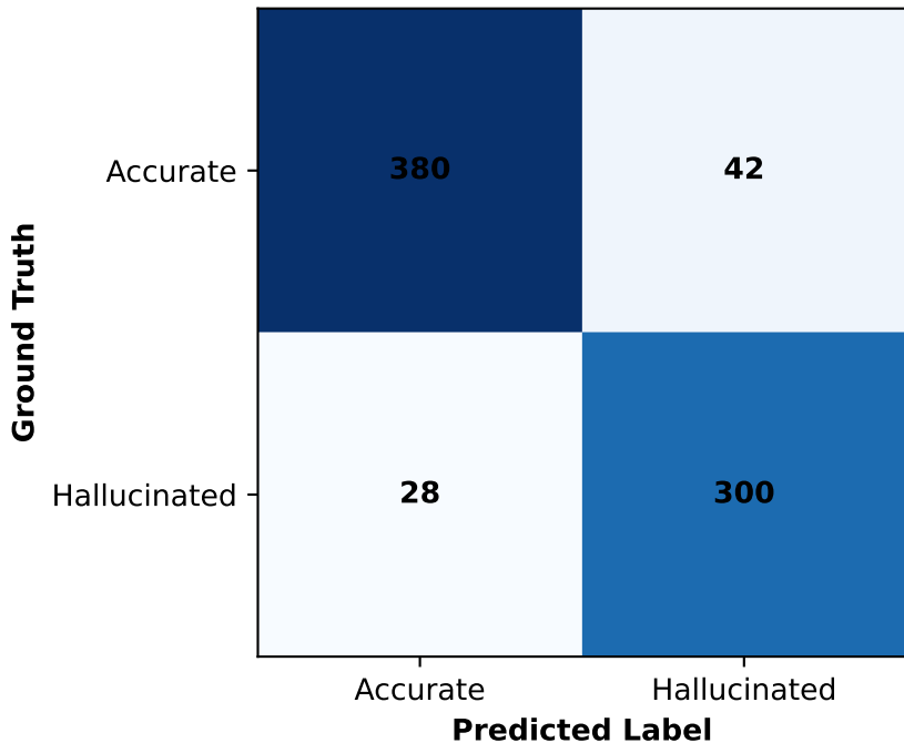
Confusion Matrix — EXP0011
