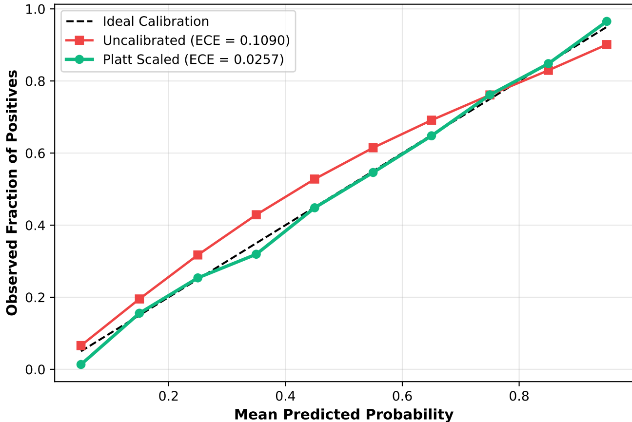
Reliability Diagram — EXP0012
