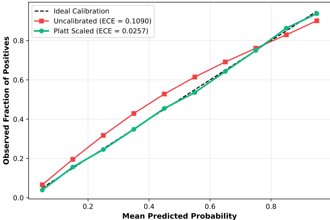
Reliability Diagram — EXP0013
