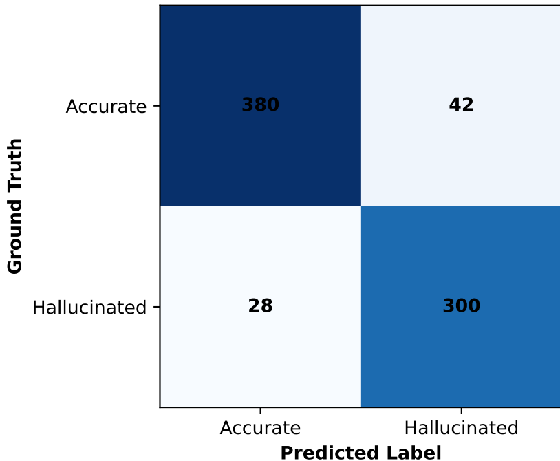
Confusion Matrix — EXP0014
