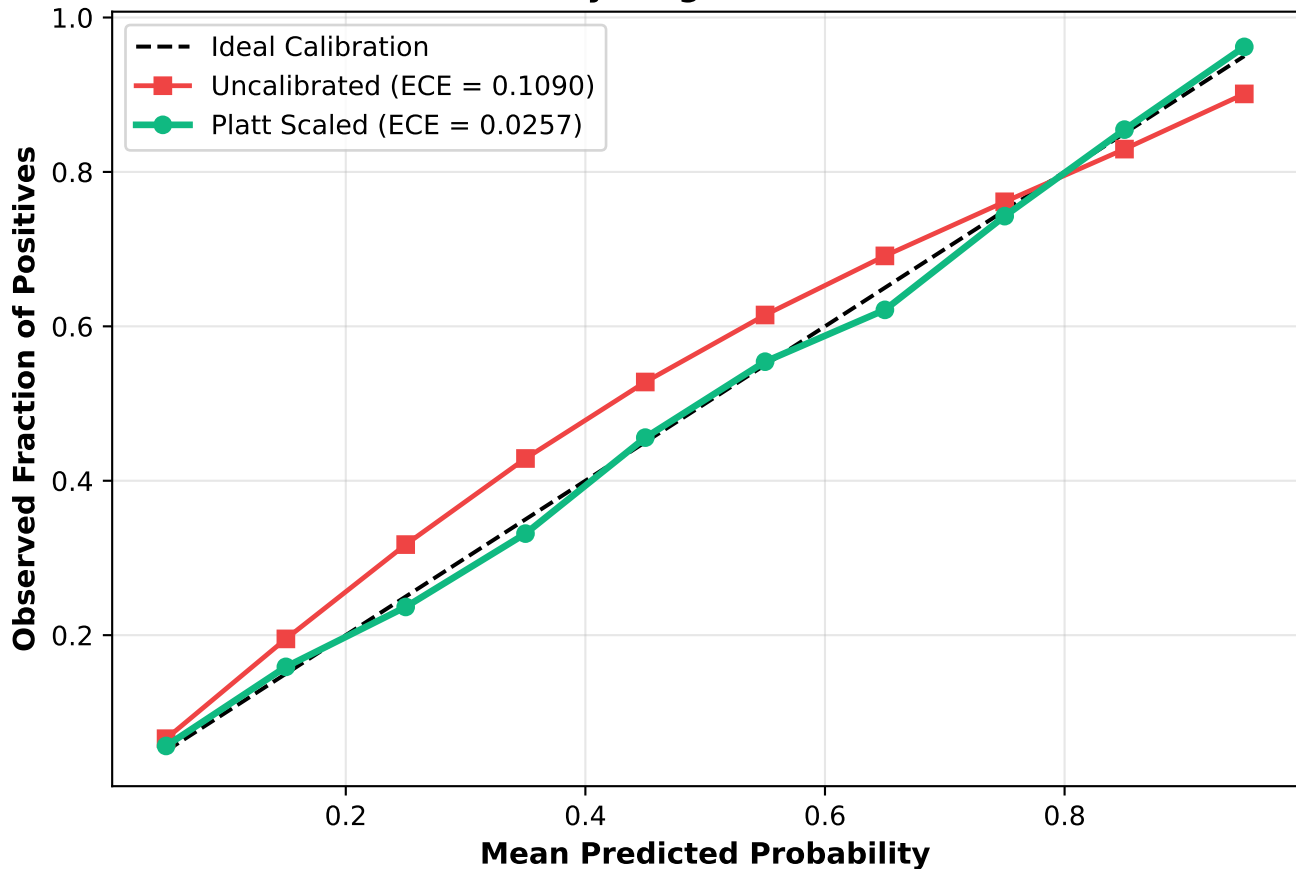
Reliability Diagram — EXP0014
