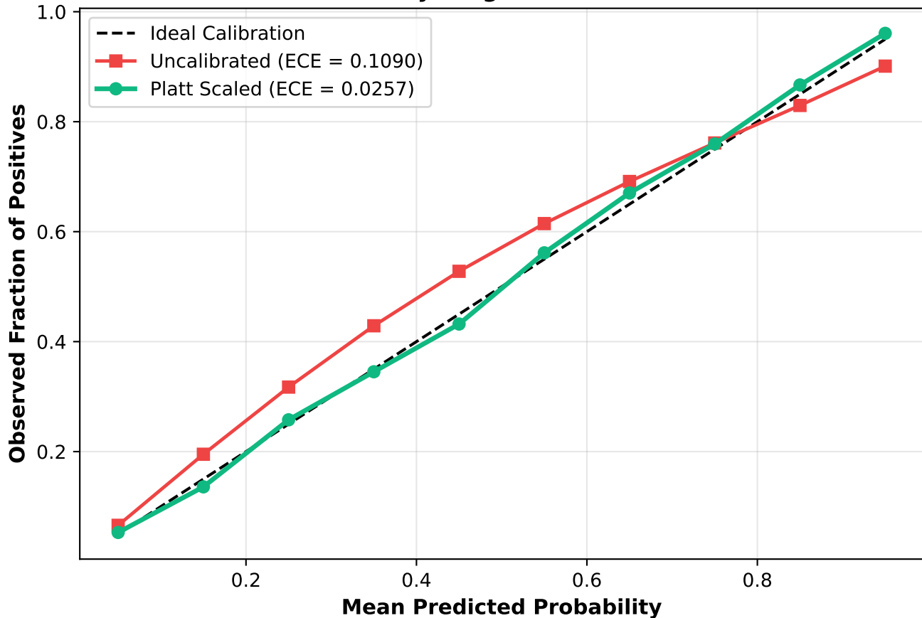
Reliability Diagram — EXP0001
