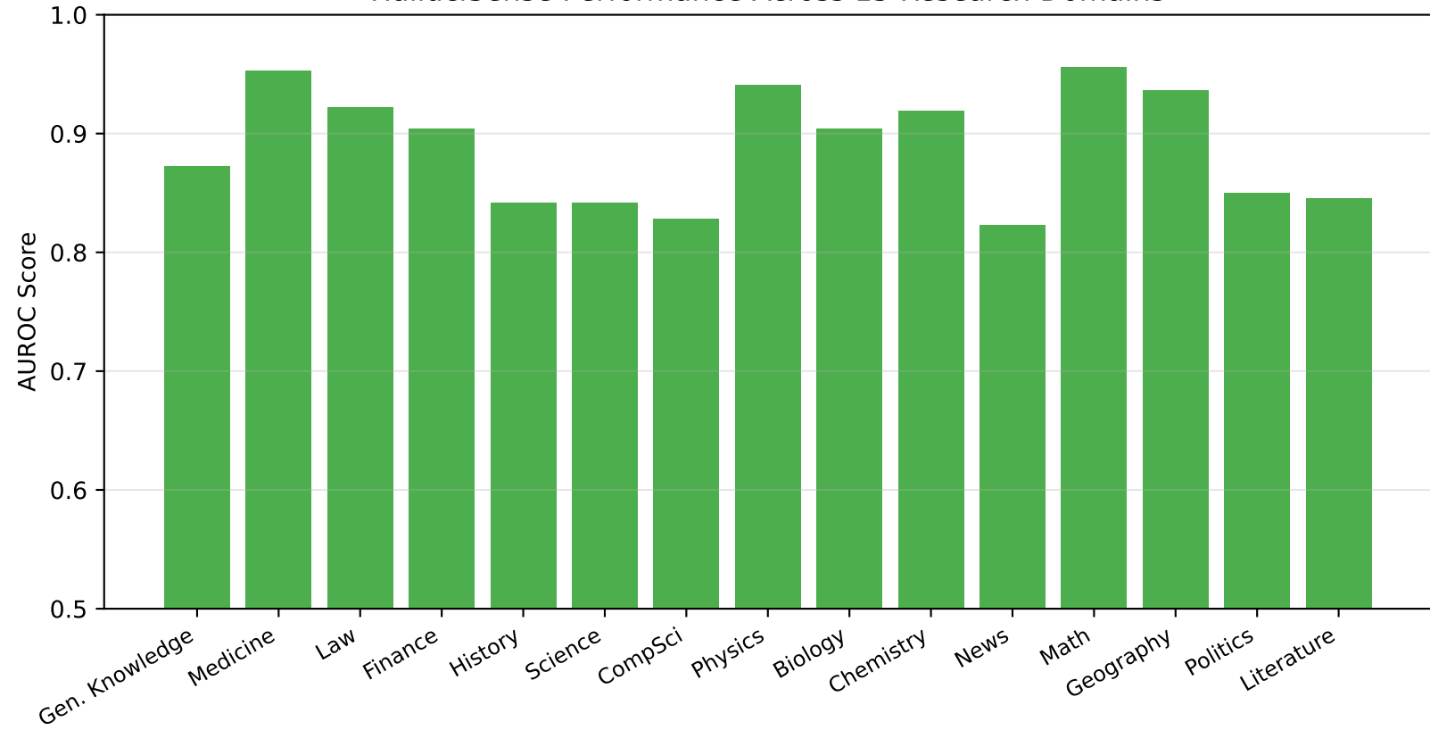
HalluciSense Performance Across 15 Research Domains
