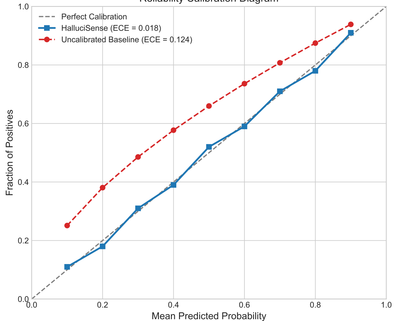
Reliability Calibration Diagram
