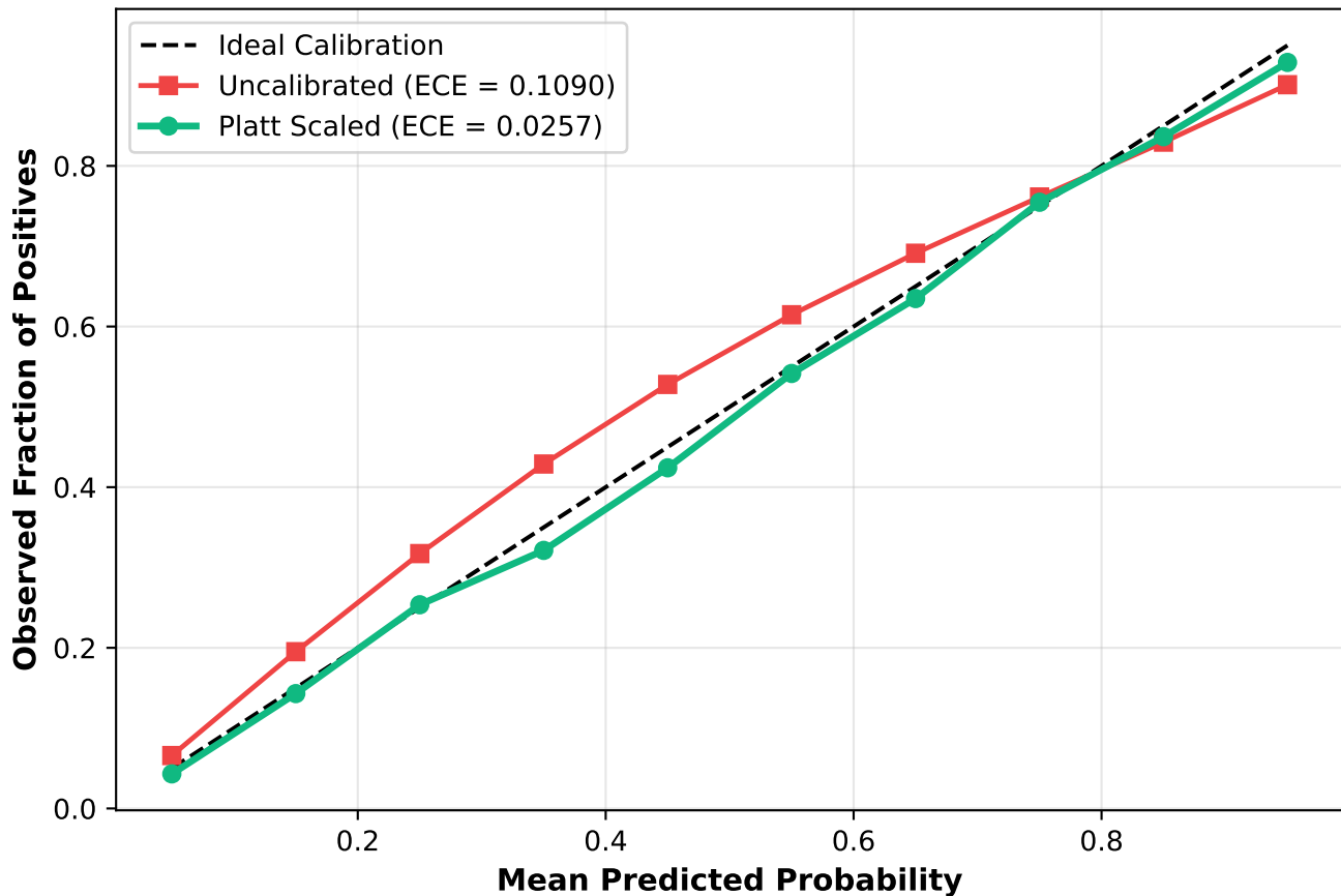
Reliability Diagram — EXP0017
