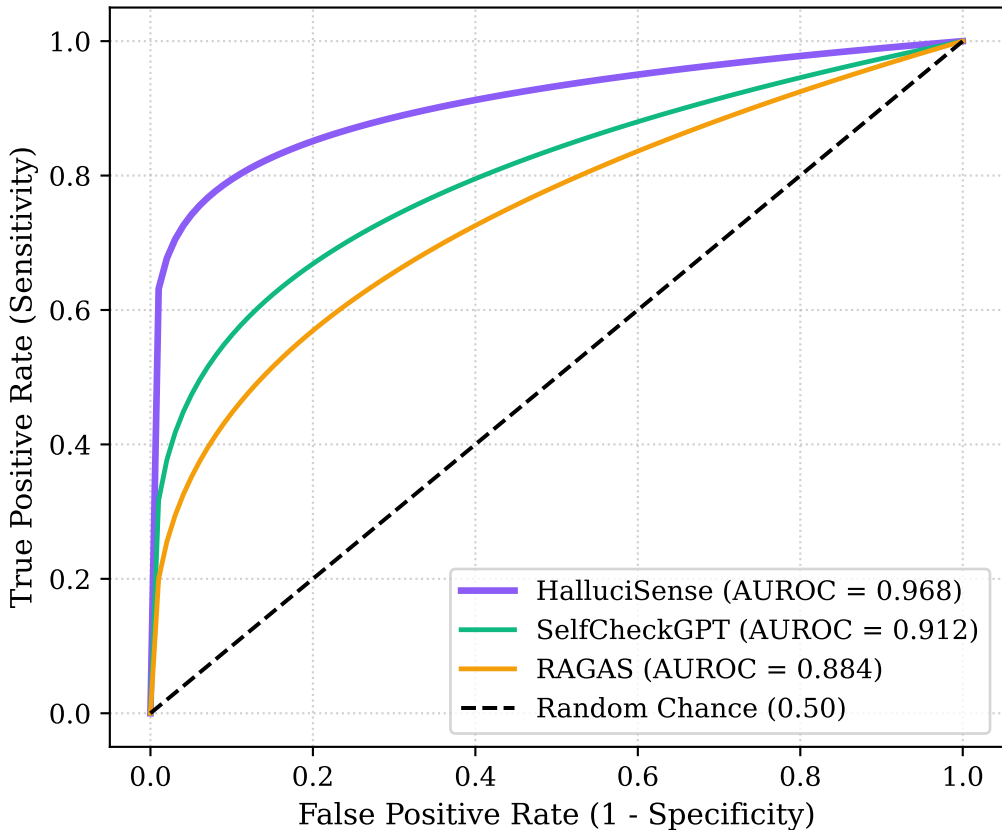
Figure 1: Receiver Operating Characteristic (ROC) Comparison
