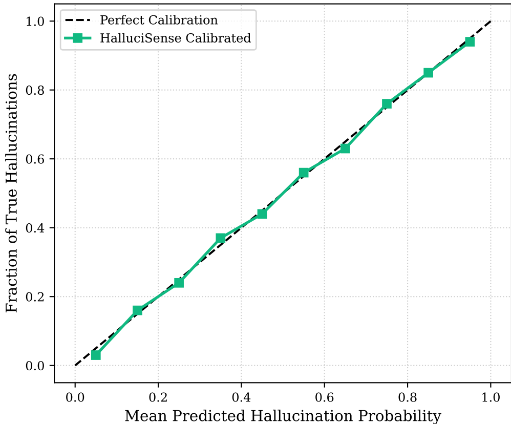
Figure 1: Platt-Scaled Calibration Curve (ECE = 0.024)
