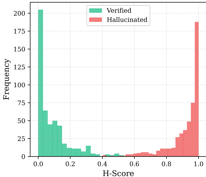
(a) H-Score Distribution
