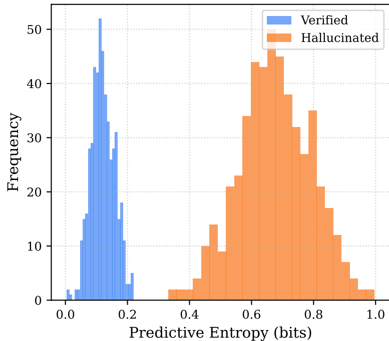
(b) Predictive Entropy Distribution
