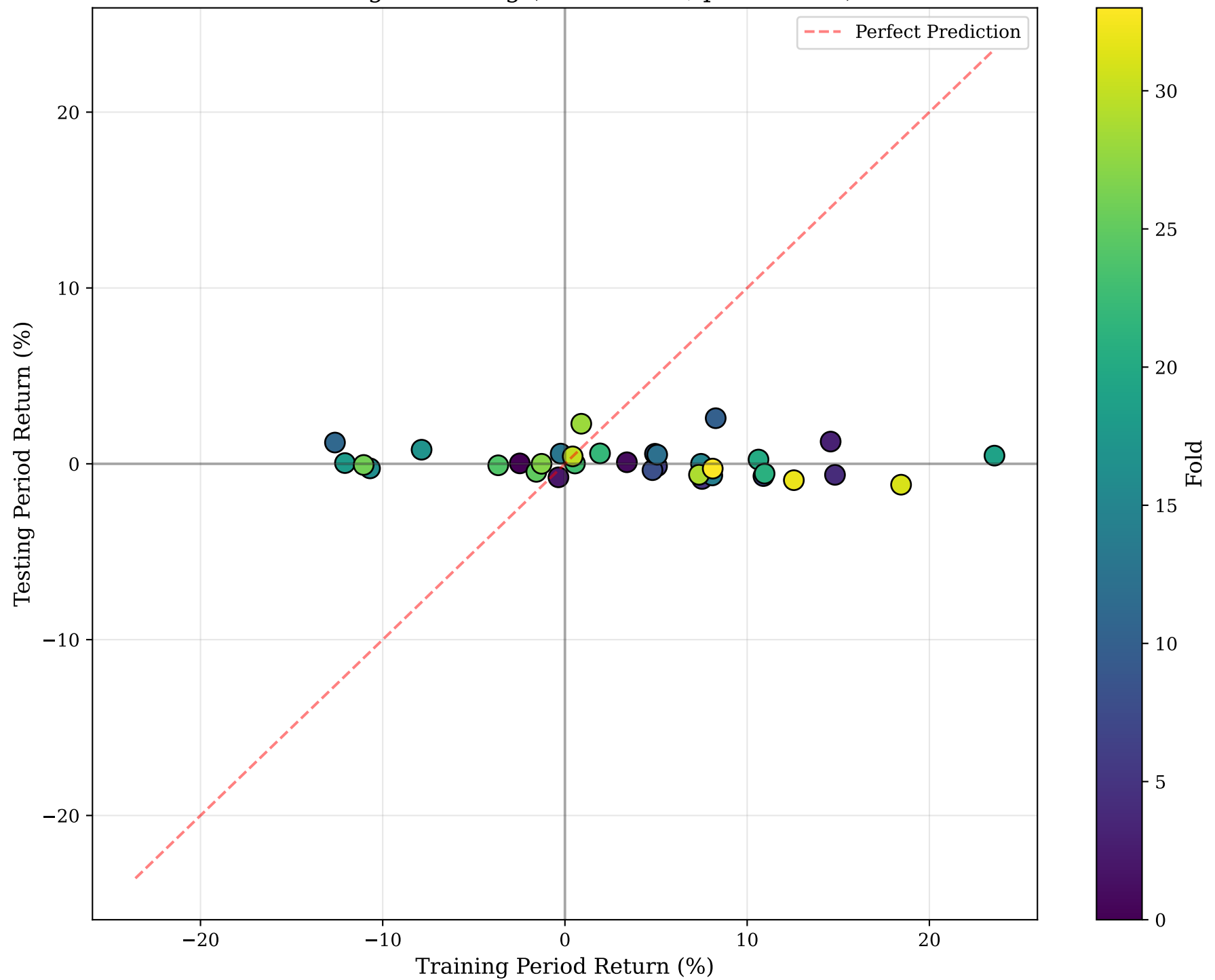
Training vs Testing (IC = -0.185, p = 0.2953)
