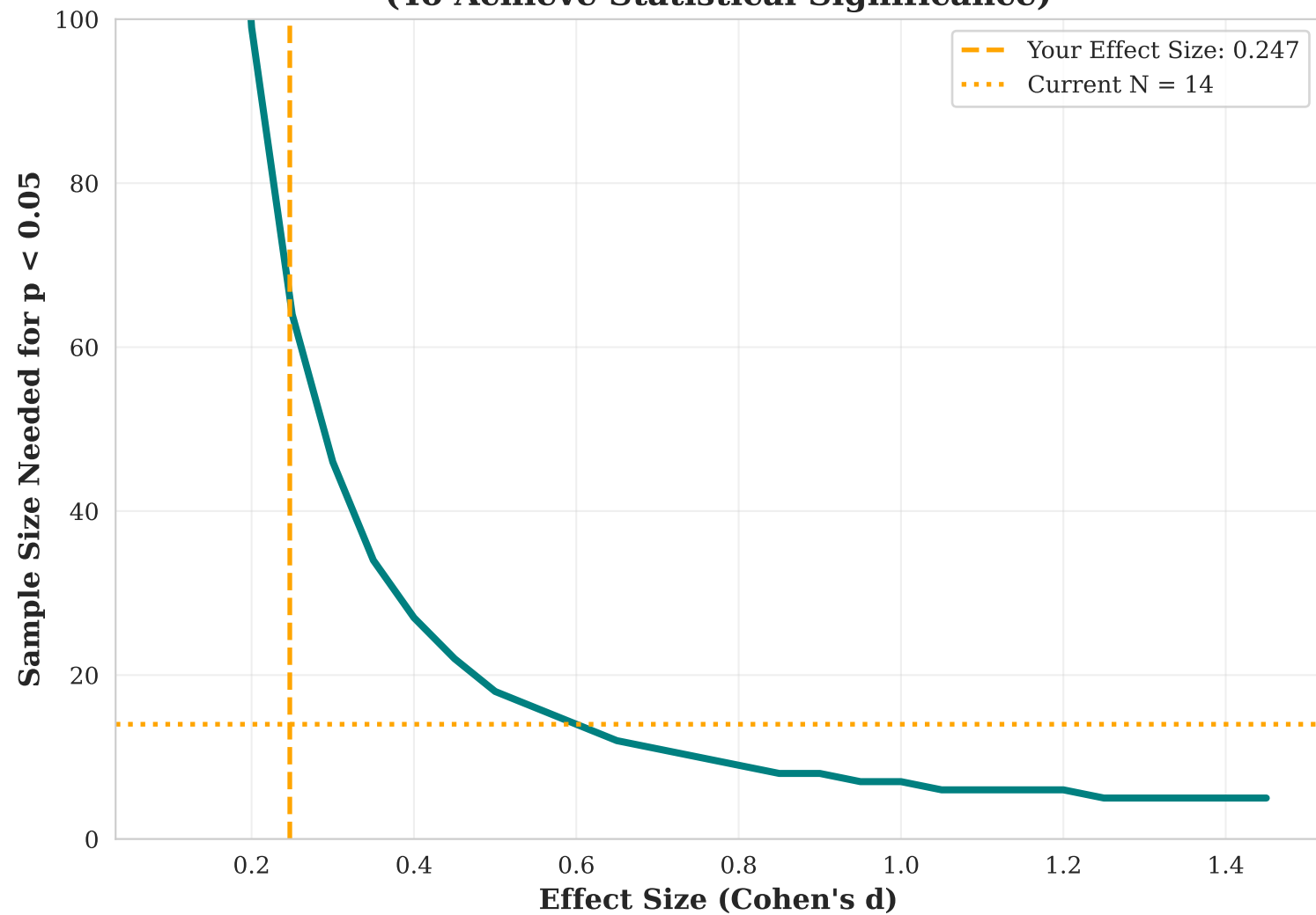
(D) Required Sample Size vs Effect Size (To Achieve Statistical Significance)
