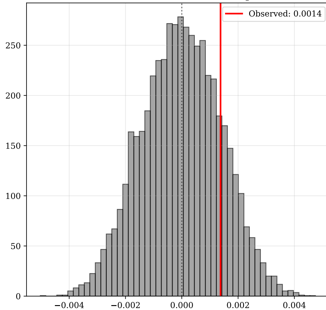
(B) Monte Carlo Permutation Test ( p = 0.3463 )
