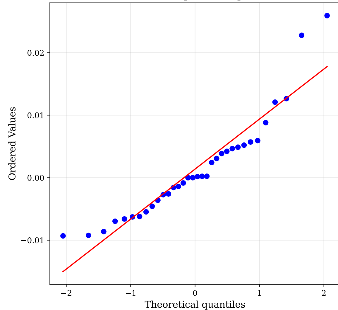
(C) Q-Q Plot (Shapiro-Wilk p = 0.0043 )
