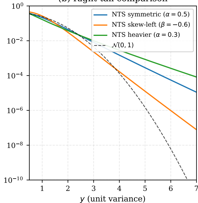
(b) Right-tail comparison
