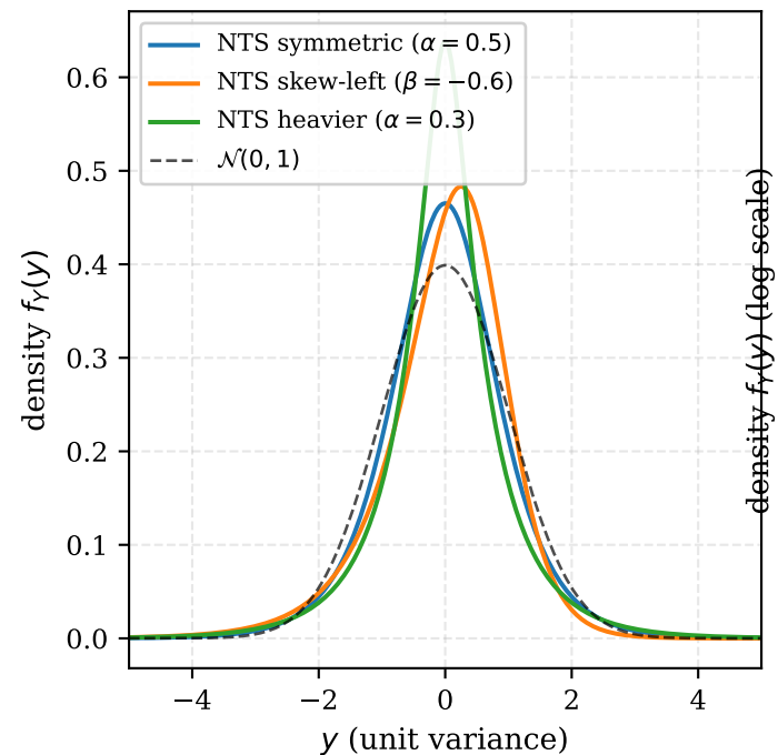
(a) NTS densities, unit variance
