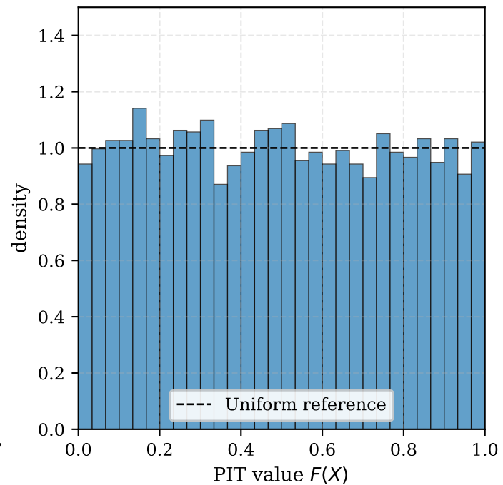
(c) PIT of n = 5000 NTS samples
